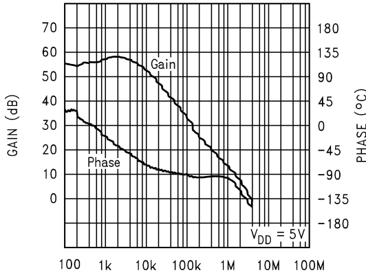
Open Loop Frequency Response, 5V
